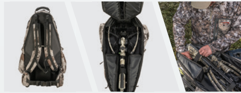
HCA-20120 HALO Bowpack - Custom Designed for TenPoint's Havoc R5440, Siege R5410, Siege 425, Flatline 460, TRX 26, TX 28, & TX 440 DIMENSIONS: Pack Length: 30" | Pack Width 15.5" | Pack Depth 11"
